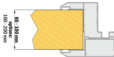
Horizontal section of the aluminum frame that covers the panel
