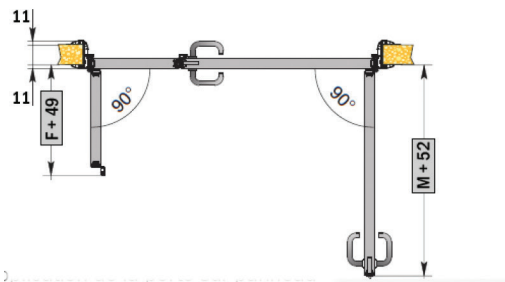
Door installation on panel
