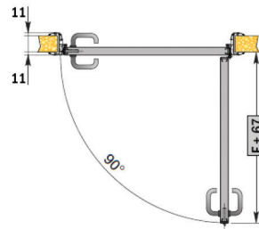
Door installation on panel
